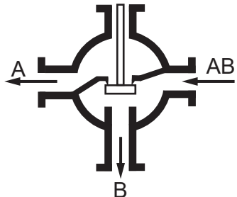
Diverting - Pressure at 'AB' Connected to 'B' 'A' Port is Close.
