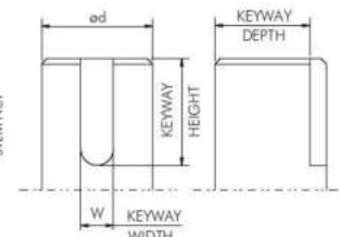
STEM END DETAILS FOR ACTUATOR/GEAR OPERATOR VALVE
