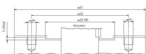
MOUNTING DETAILS OF ACTUATOR/GEAR OPERATOR AS PER ISO-5211
